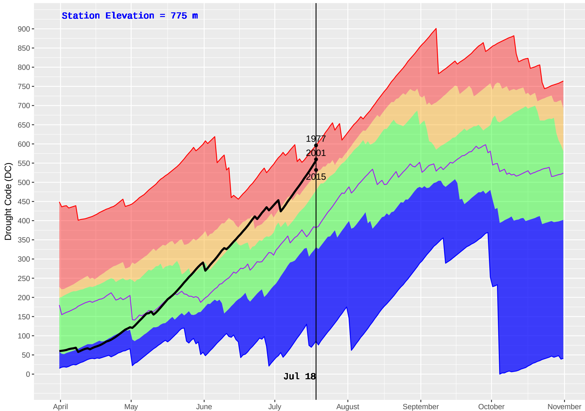
ELKO (412) : Historical (1970–2016) and Current (2018) Daily Drought Code (DC)
